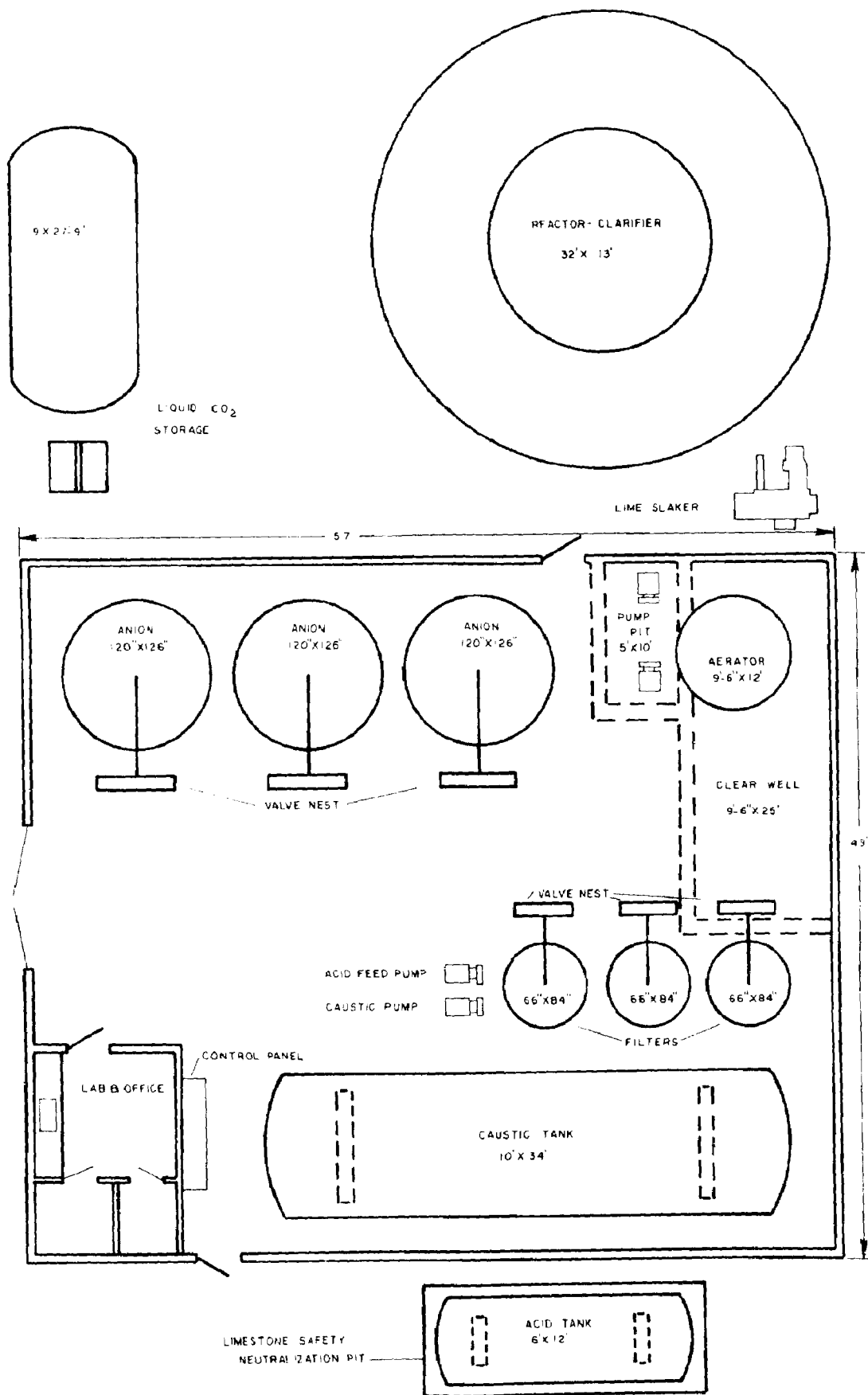
FIGURE 30. AMD Treatment Plant Plan, Modified Desal System 1.0 MGD
