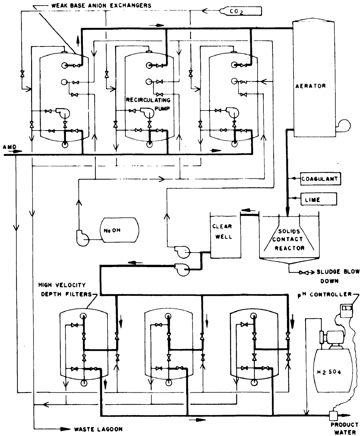
FIGURE 29. AMD Treatment Plant Flow Desal System 1.0 MGD
